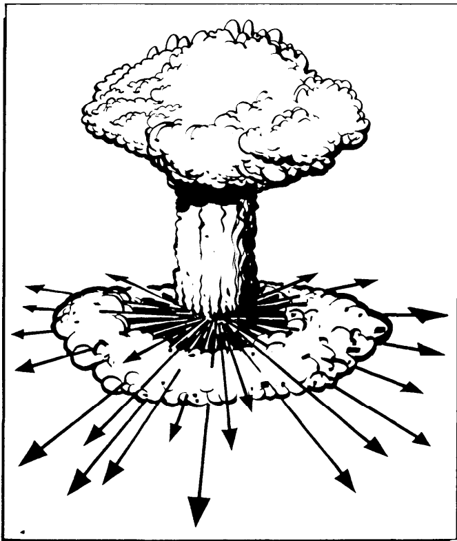
Figure 29-5. Nuclear Radiation.
