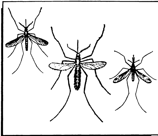
Figure 30-1. Vectors.
